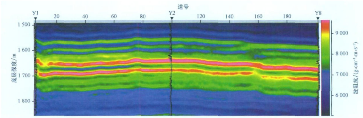
图 4 连井的波阻抗反演剖面 Fig. 4 Acoustic impedance inversion section with three wells tied
