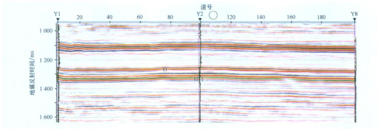
图 2 连井地震剖面 Fig. 2 Seismic section with three wells tied
