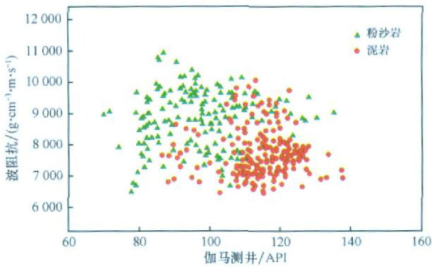
图 3 波阻抗与岩性交汇图 Fig. 3 Cross plot of impedance and lithology
